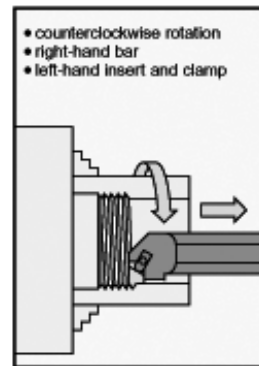
internal left-hand thread
