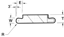
FLR (RH Shown)
