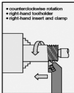
external right-hand thread
