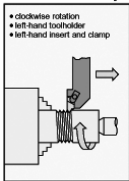
external right-hand thread
