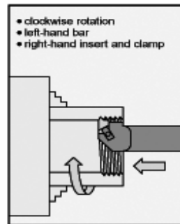
internal left-hand thread
