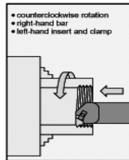
internal right-hand thread
