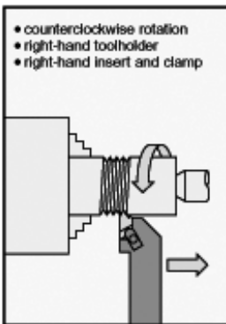
external left-hand thread
